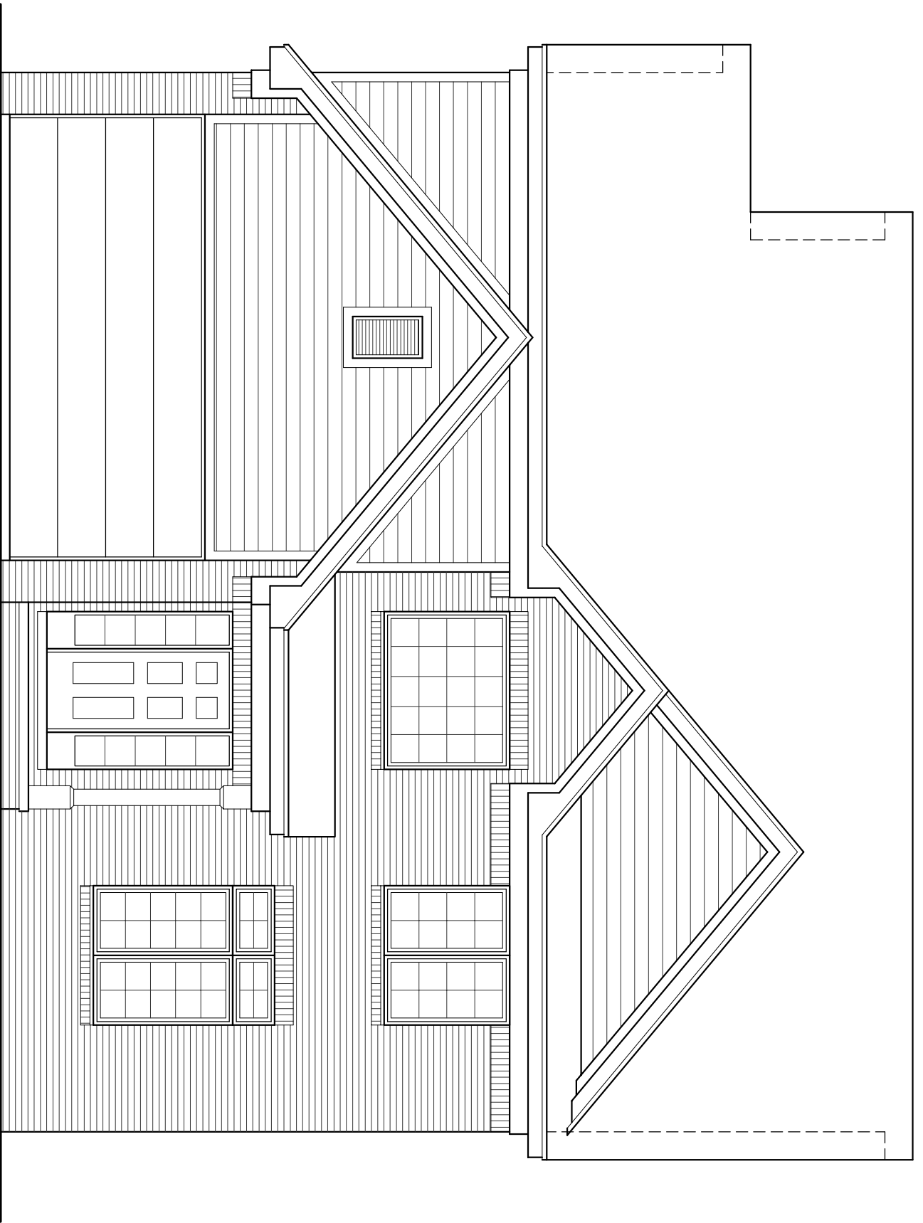
front elevation
